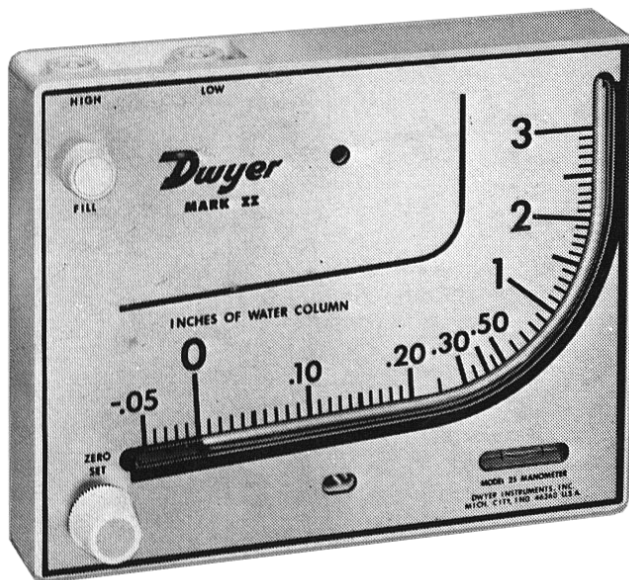
Mark II molded plastic incline air filter gage.
