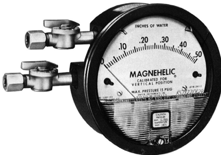
Dial type Series 2000 Magnehelic® air filter gage.
