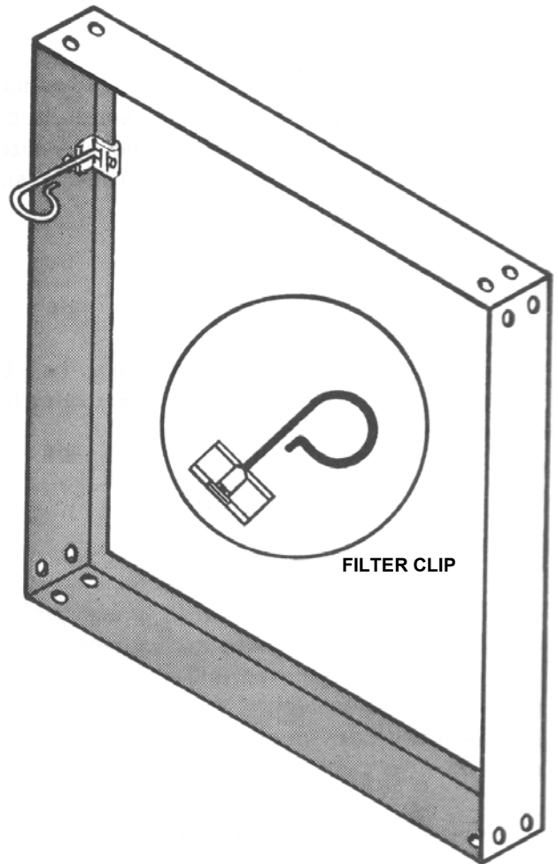
UTILITY FRAME
