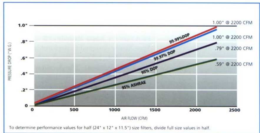
AIR FLOW VS. PRESSURE DROP
