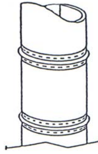
TUBULAR Anti-Collapse Rings Internal Dust Cake Used in Reverse Air Collectors
